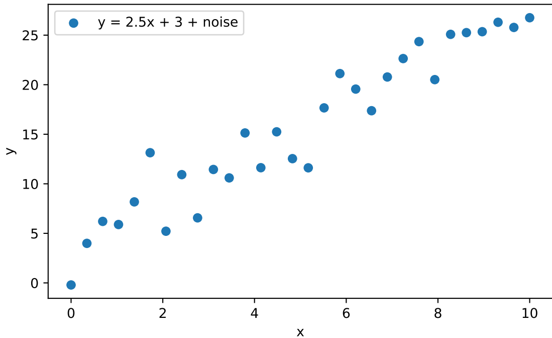
Linear fit with noise
