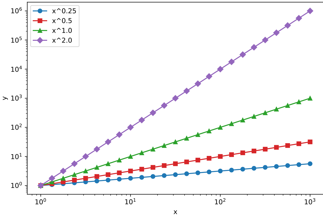
Log-log 4 power laws
