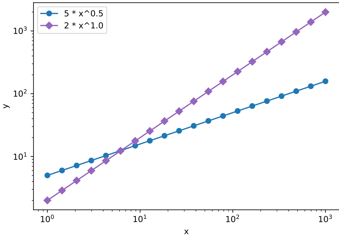
Power laws
