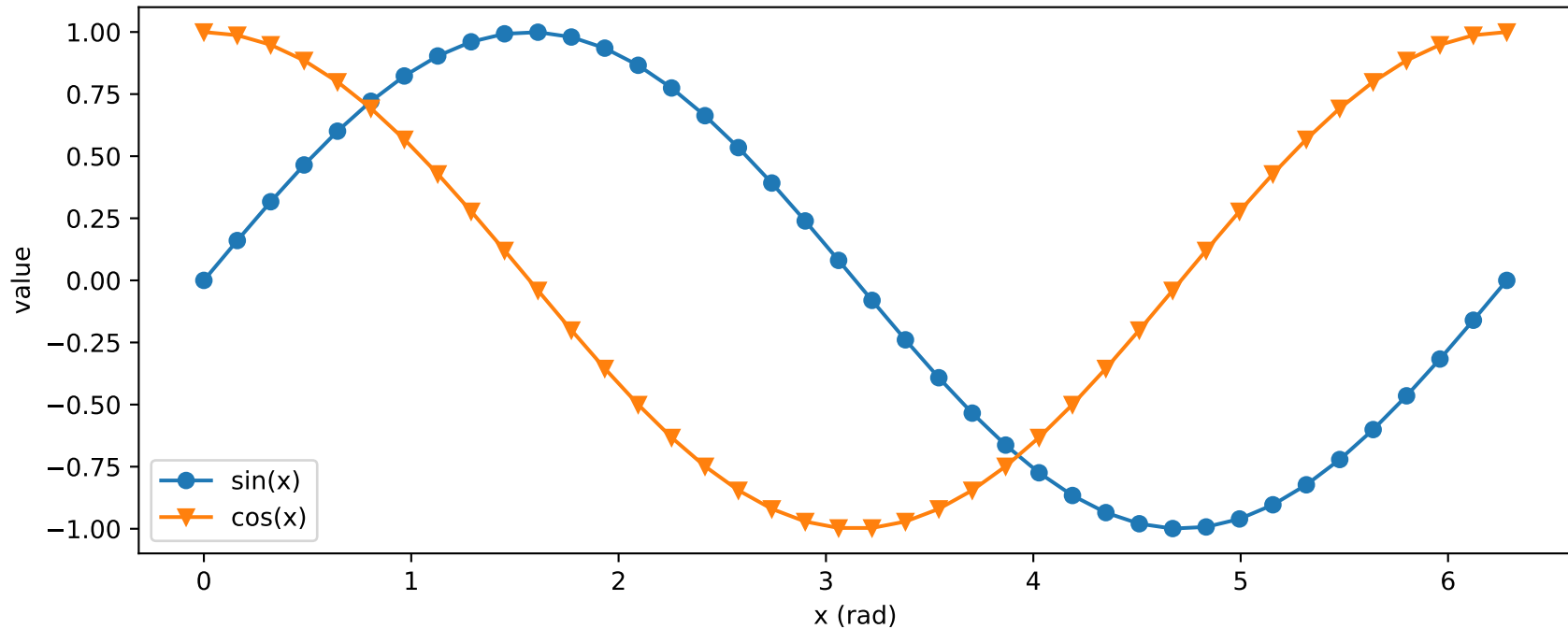
Trig functions
