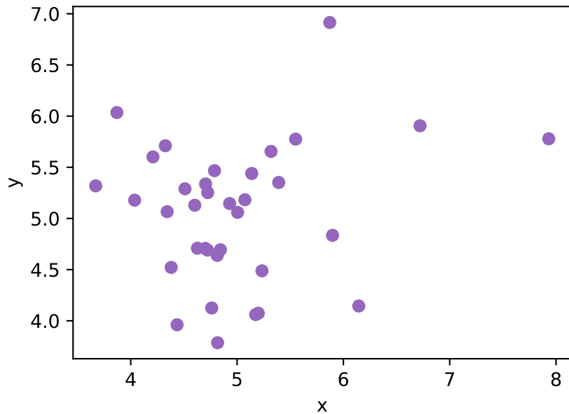
cluster
