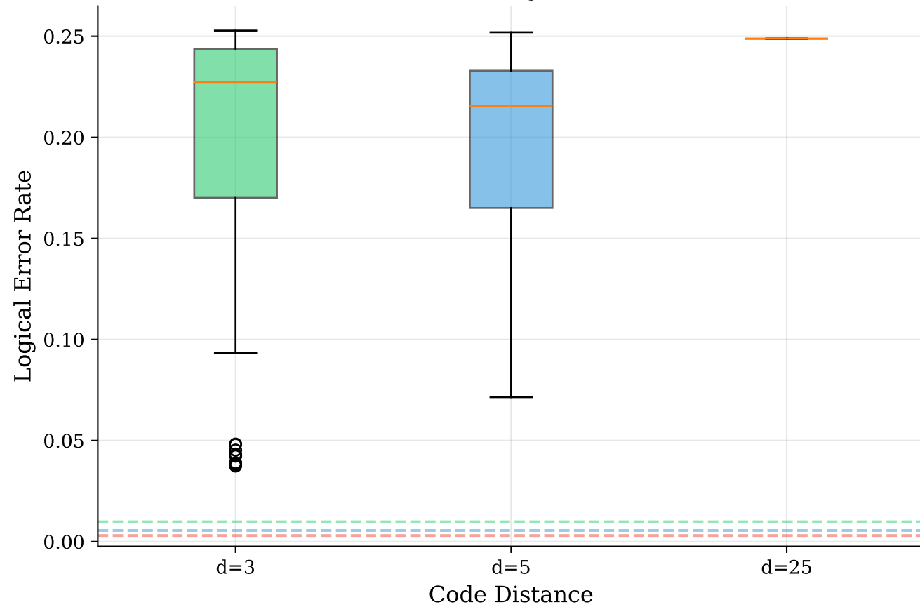
LER Distribution by Code Distance
