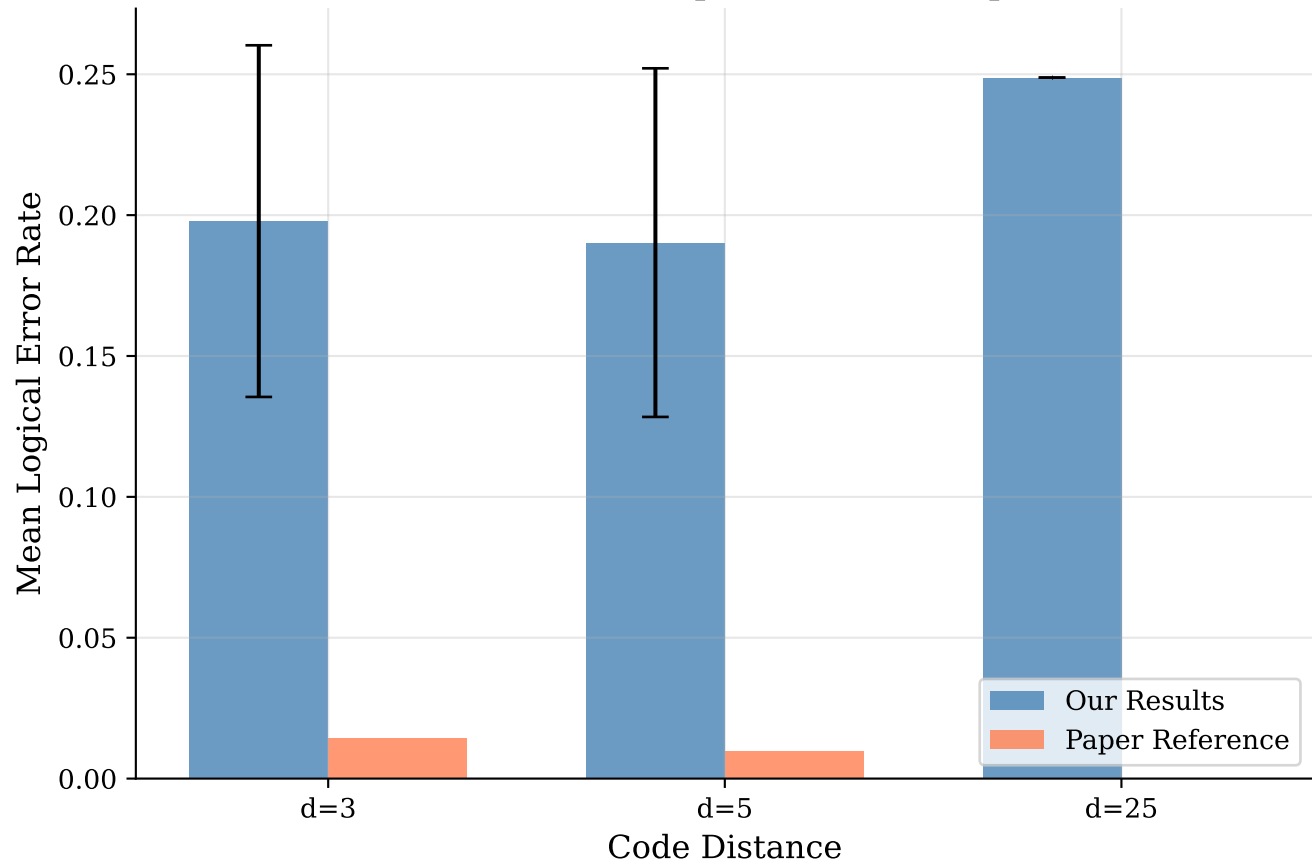
Mean LER Comparison with Paper
