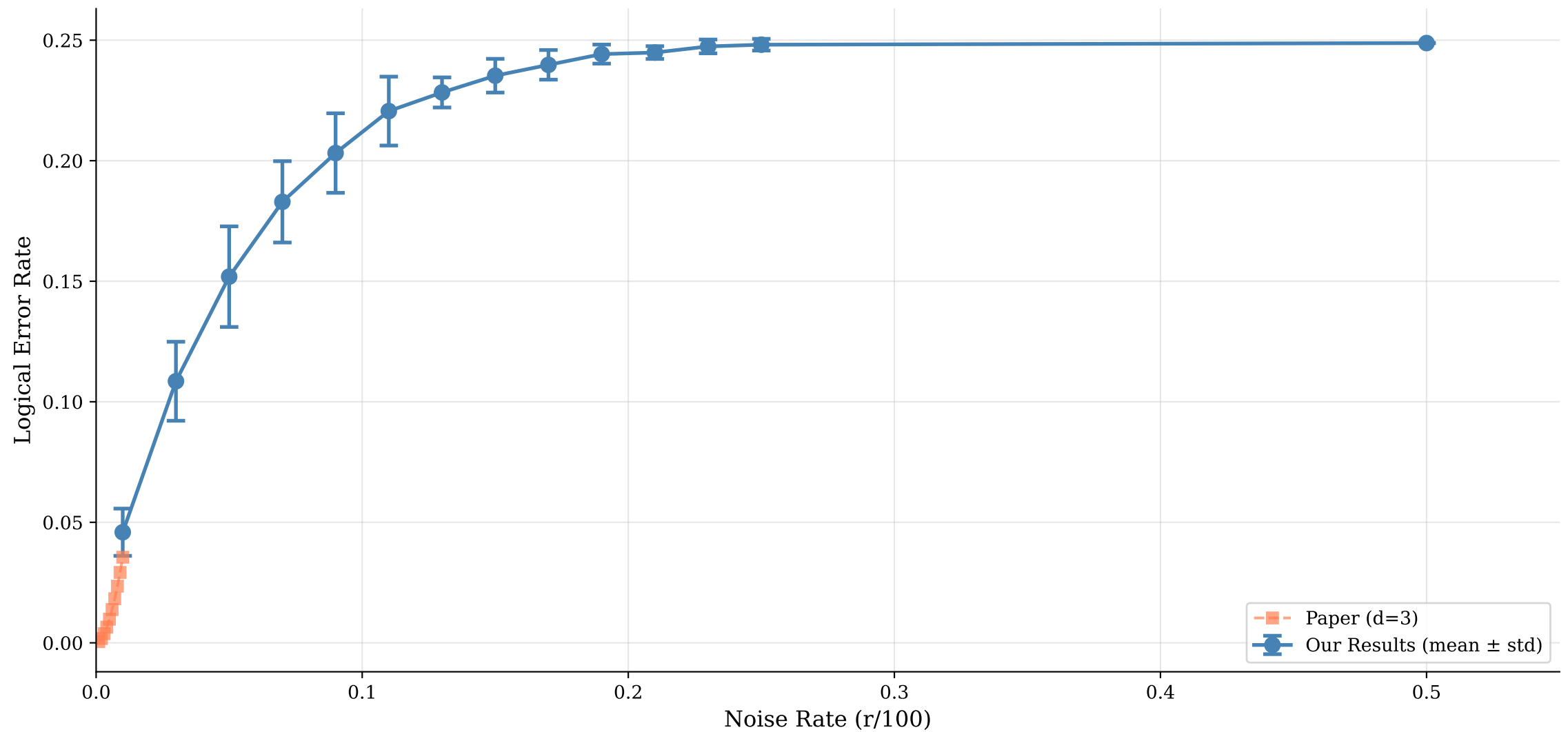
LER vs Noise Rate
