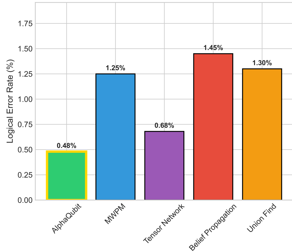
Pauli+, p=0.5\% , d=5
