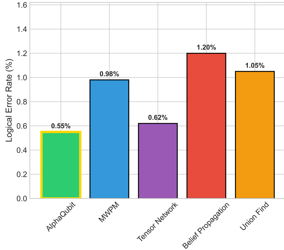
SI1000, p=0.5\% , d=5
