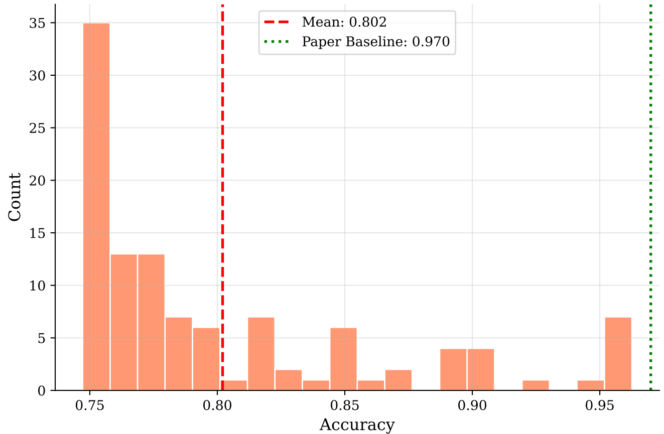
Distribution of Model Accuracies
