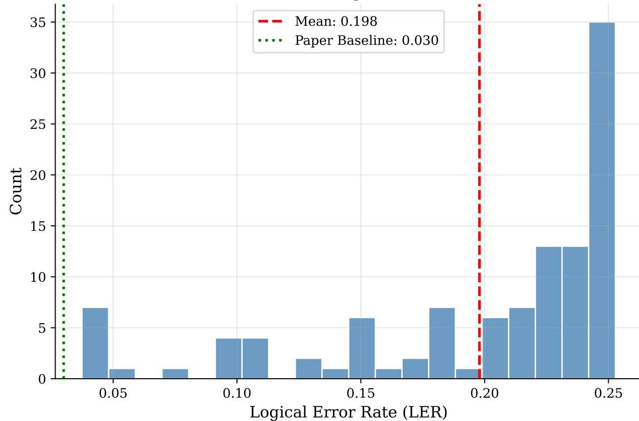
Distribution of Logical Error Rates
