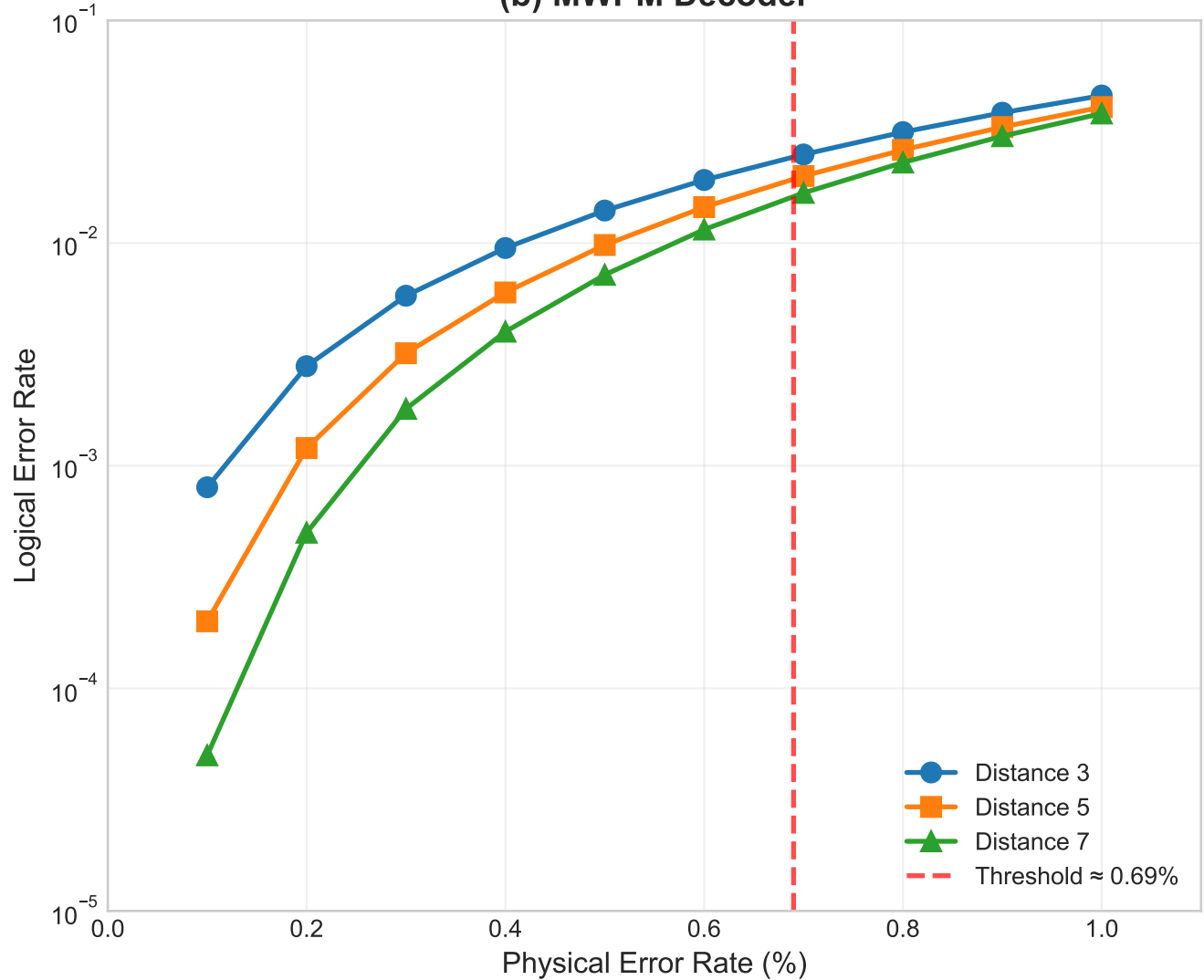
(b) MWPM Decoder
