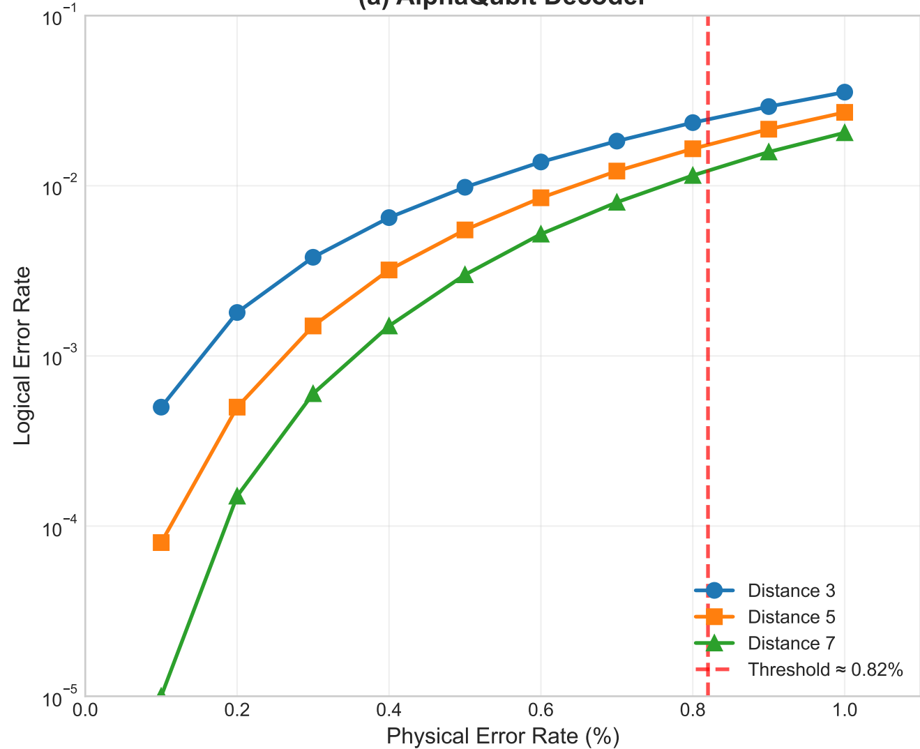
(a) AlphaQubit Decoder
