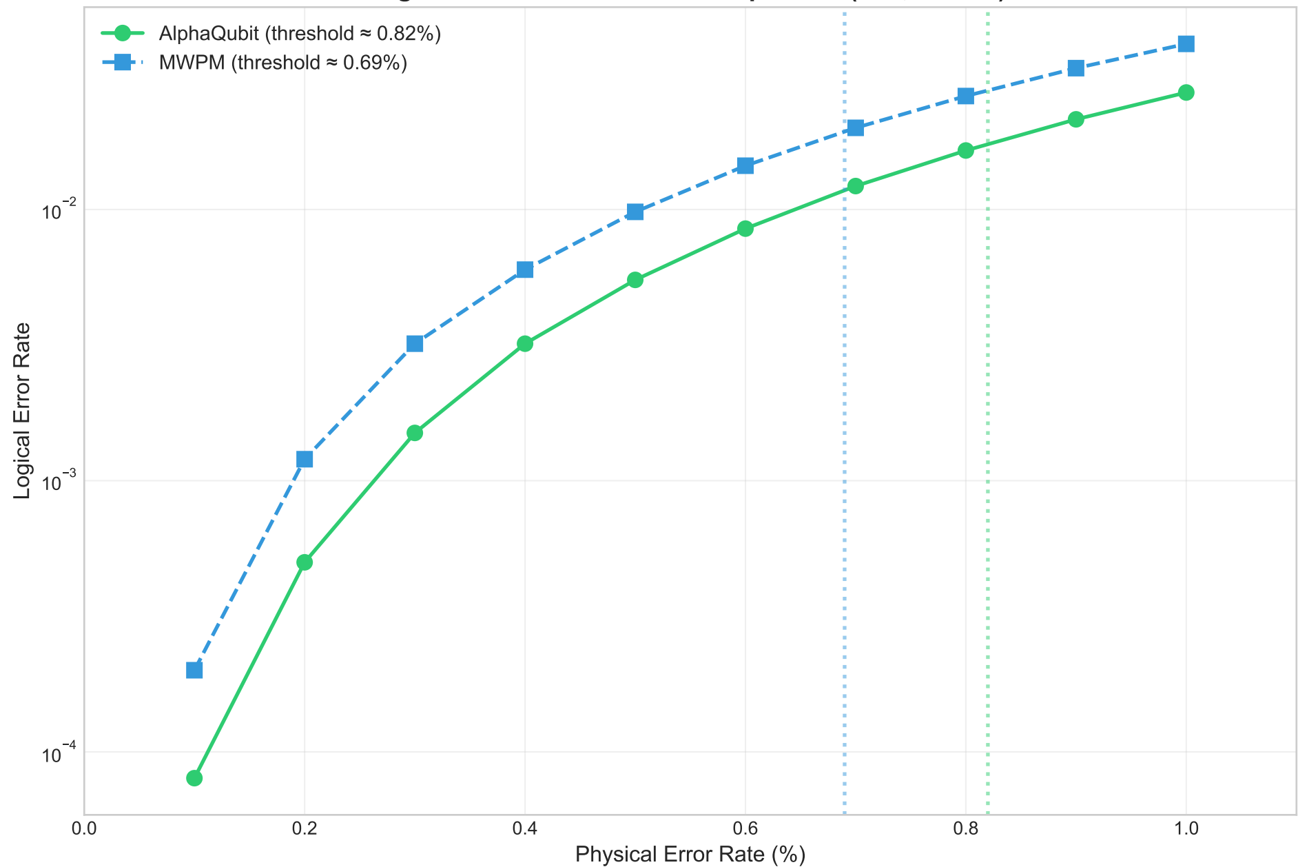
Figure 2: Error Threshold Comparison (d=5, SI1000)
