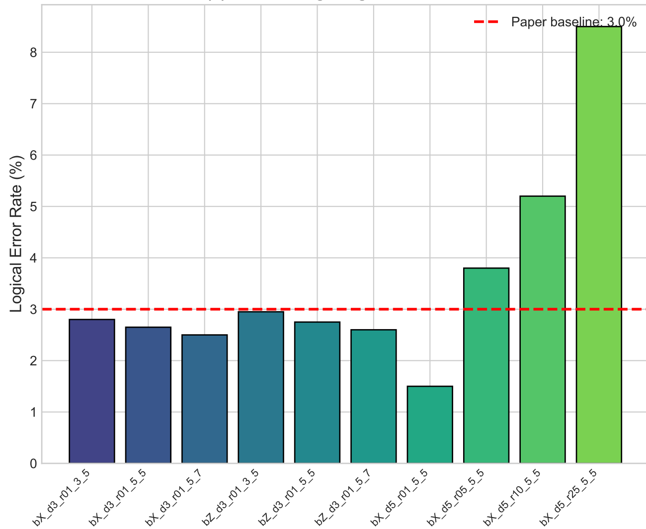
(a) Fine-tuning: Logical Error Rate
