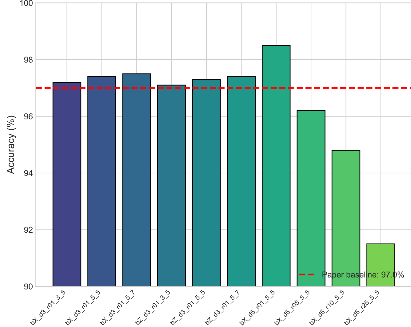
(b) Fine-tuning: Accuracy
