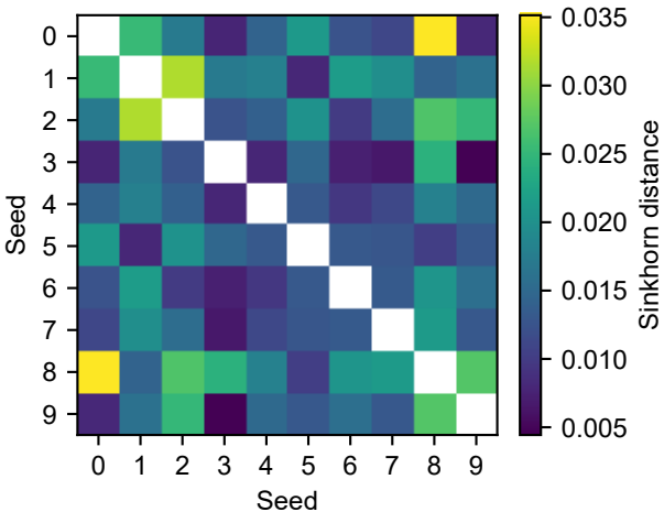
CRISP
