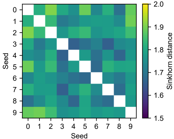
DiffCRISP
