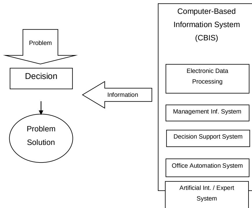
Gambar 2.3 Model CBIS
