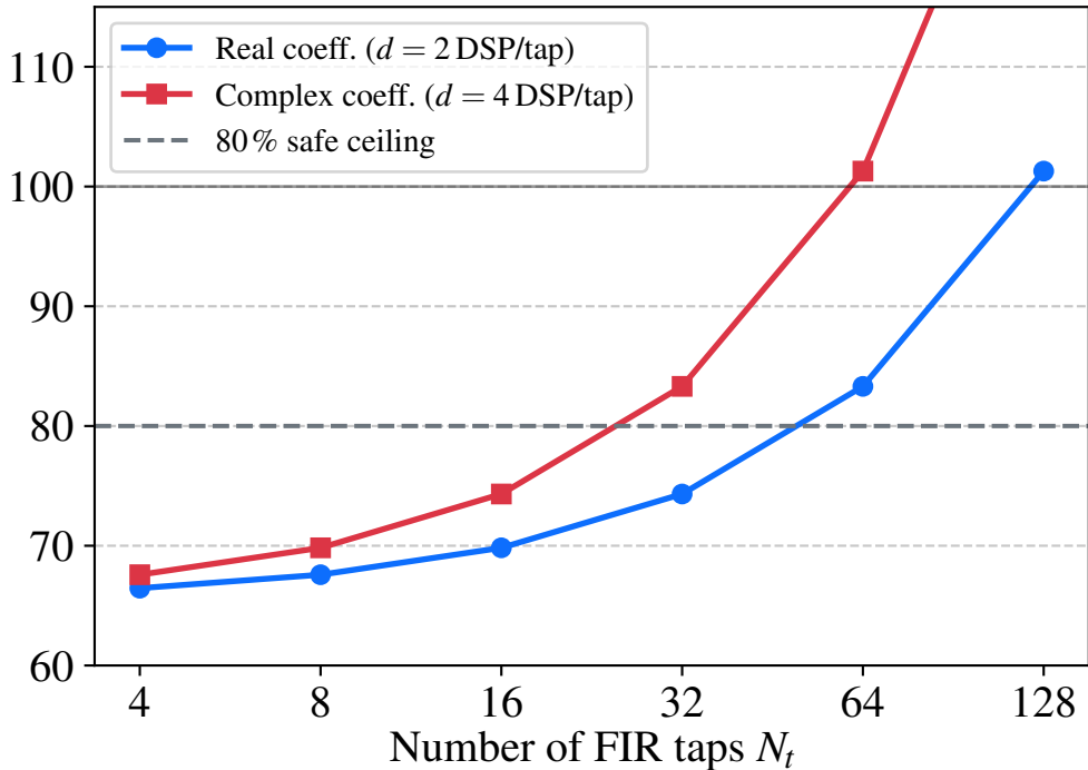
DSP48E2 utilization (%)
