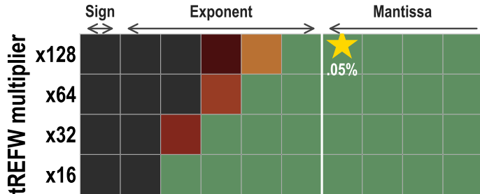
FP16 (E5M10)
