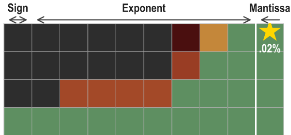
BF16 (E8M7)
