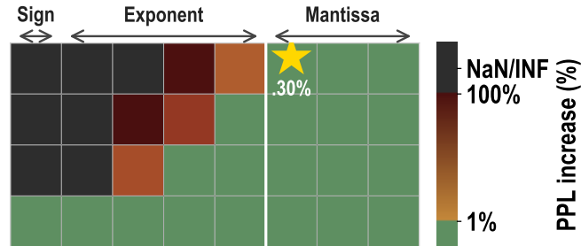
FP8 (E4M3)
