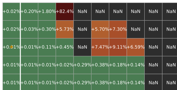
BF16 (dummy)
