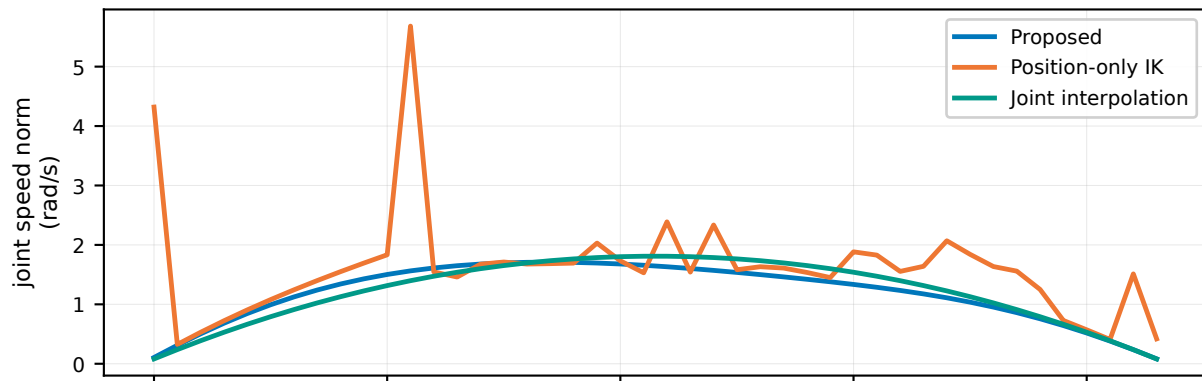
Joint-space smoothness profile, target 6
