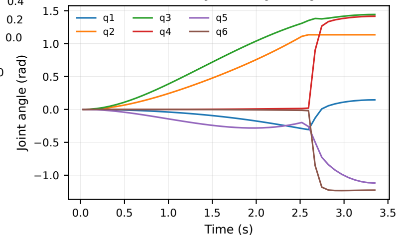
Planned joint trajectory
