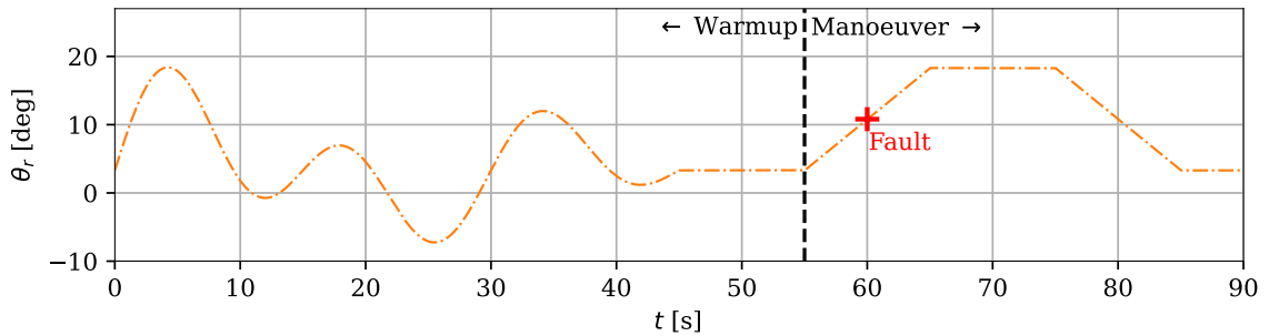
Fig. 3 Reference pitch signal \theta_r , vertical black line at 55 s demarcates the end of the warmup phase and the start of the manoeuvring phase, red cross at 60 marks introduction of fault if any.
