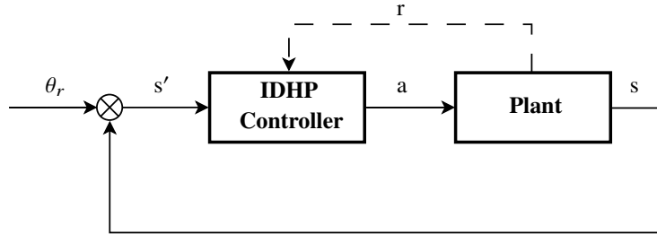
Fig. 1 Control configuration of the pitch control MDP.
