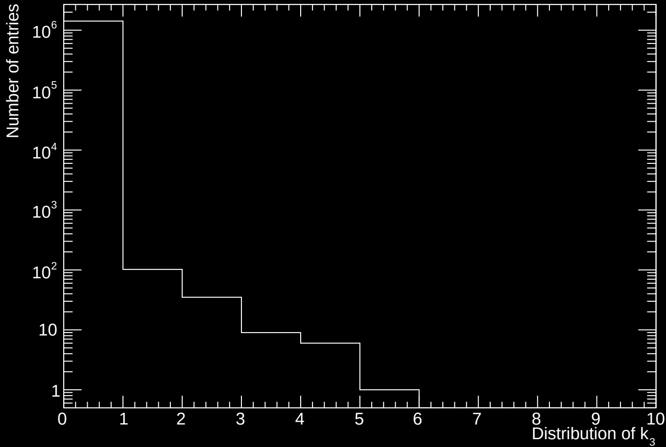
Distribution of k_3 per window
