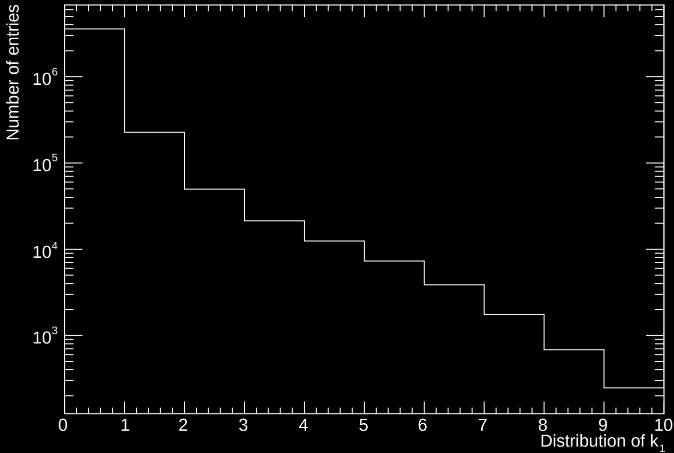
Distribution of k_1 per window
