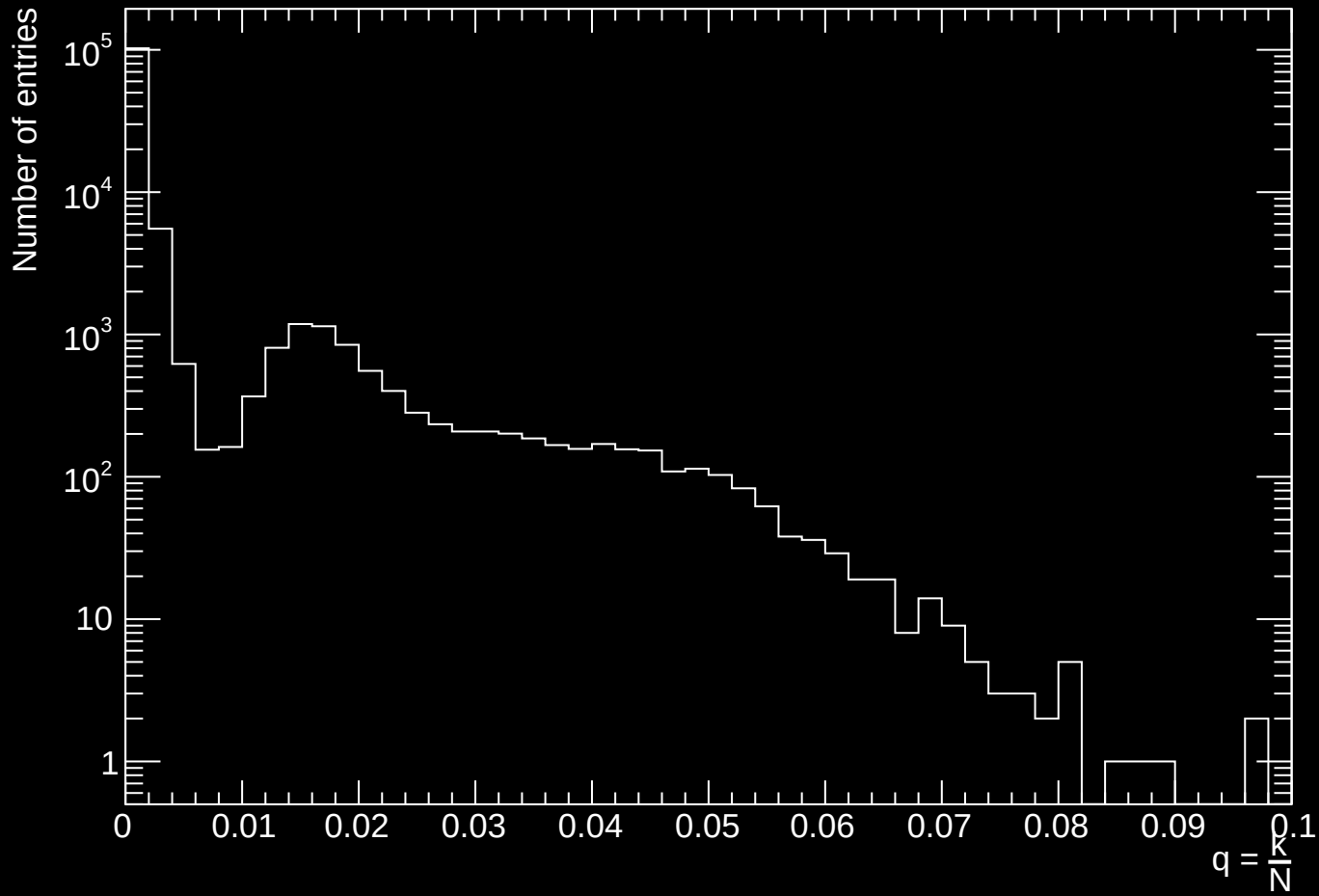
Distribution of q_1 = \frac{k}{N}
