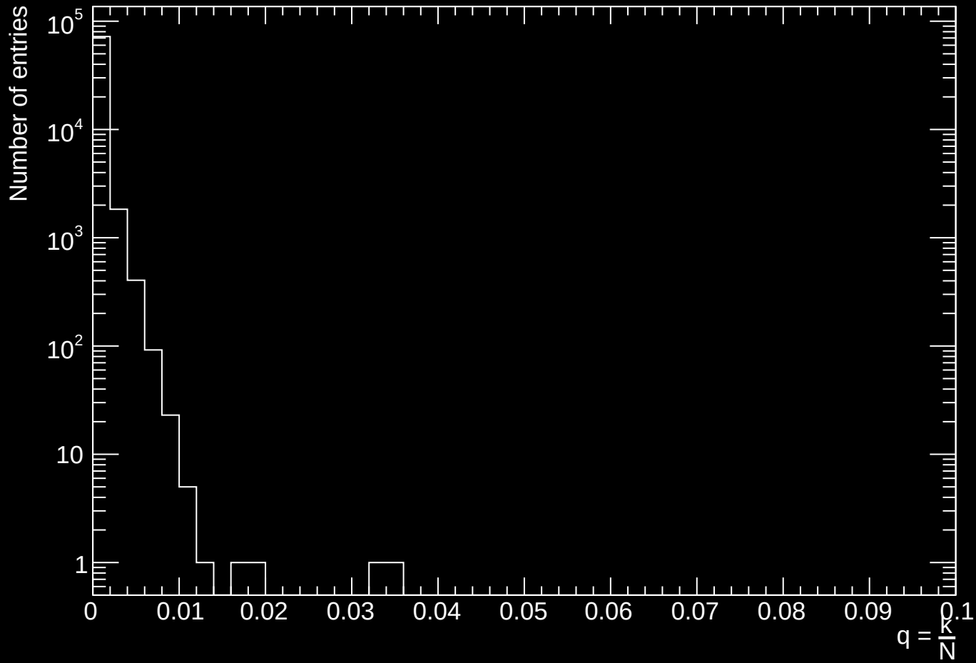
Distribution of q = \frac{k}{N}
