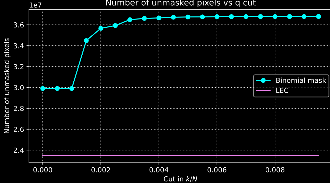
Number of unmasked pixels vs q cut
