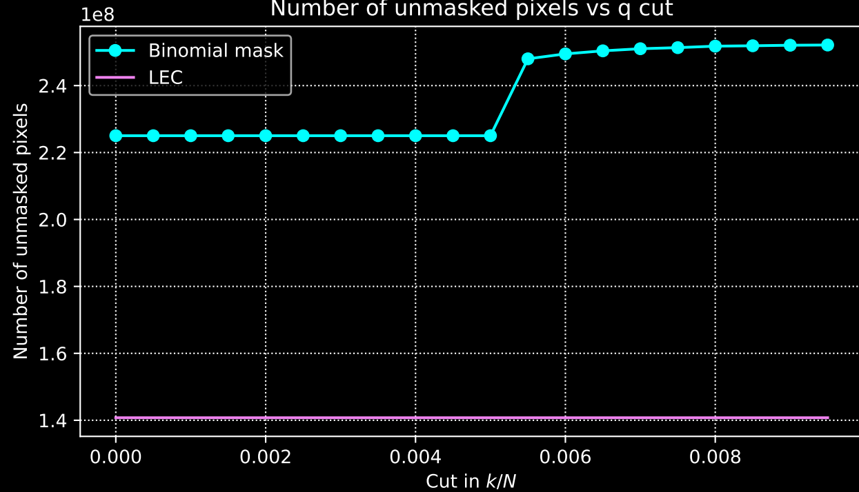
Number of unmasked pixels vs q cut
