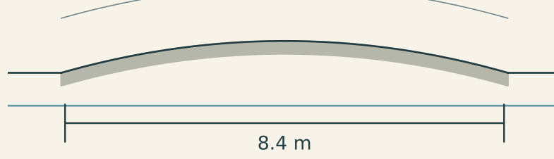
桥纵剖面补充·桥面起伏 0.6 m
