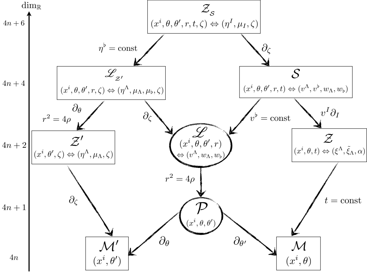
Figure 1. Overview of the QK/HK correspondence.
