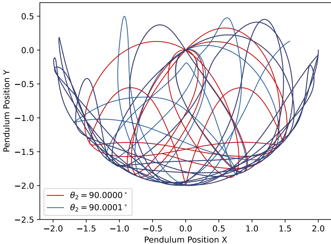
Two Slightly Different Pendula Simulation Outcome
