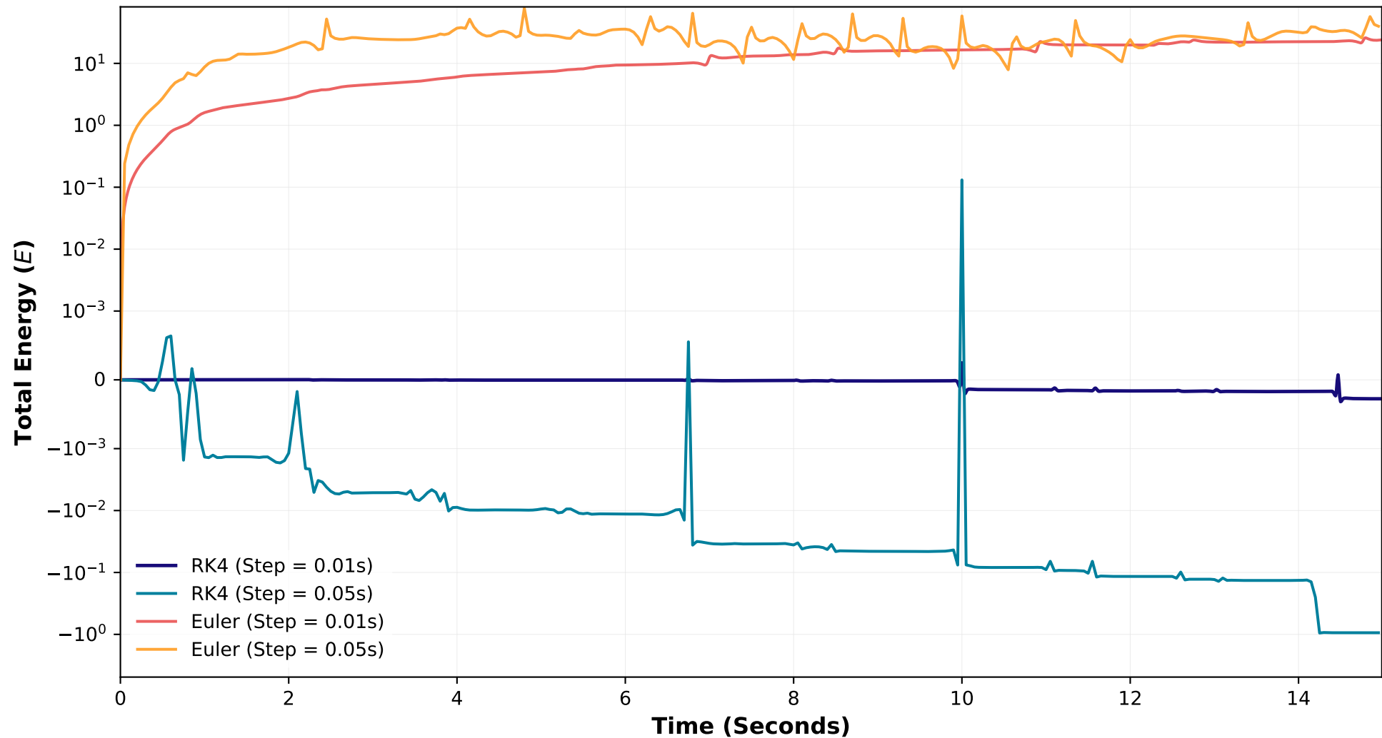
System Energy Conservation: Euler vs. RK4 Method
