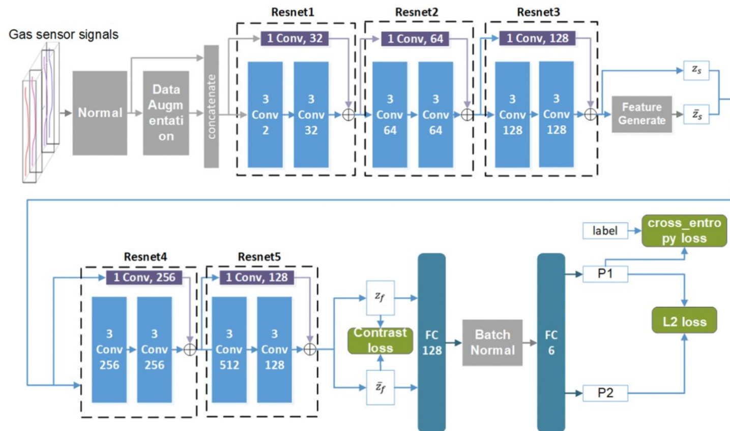
Fig. 2. The framework of CDCNN.
