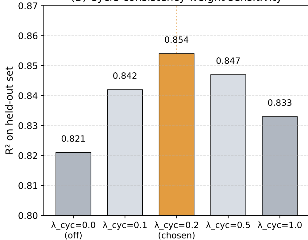
(B) Cycle-consistency weight sensitivity
