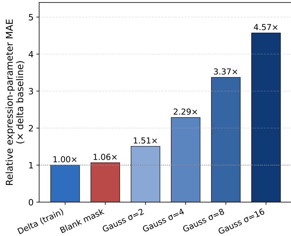
(A) Landmark-mask design ablation
