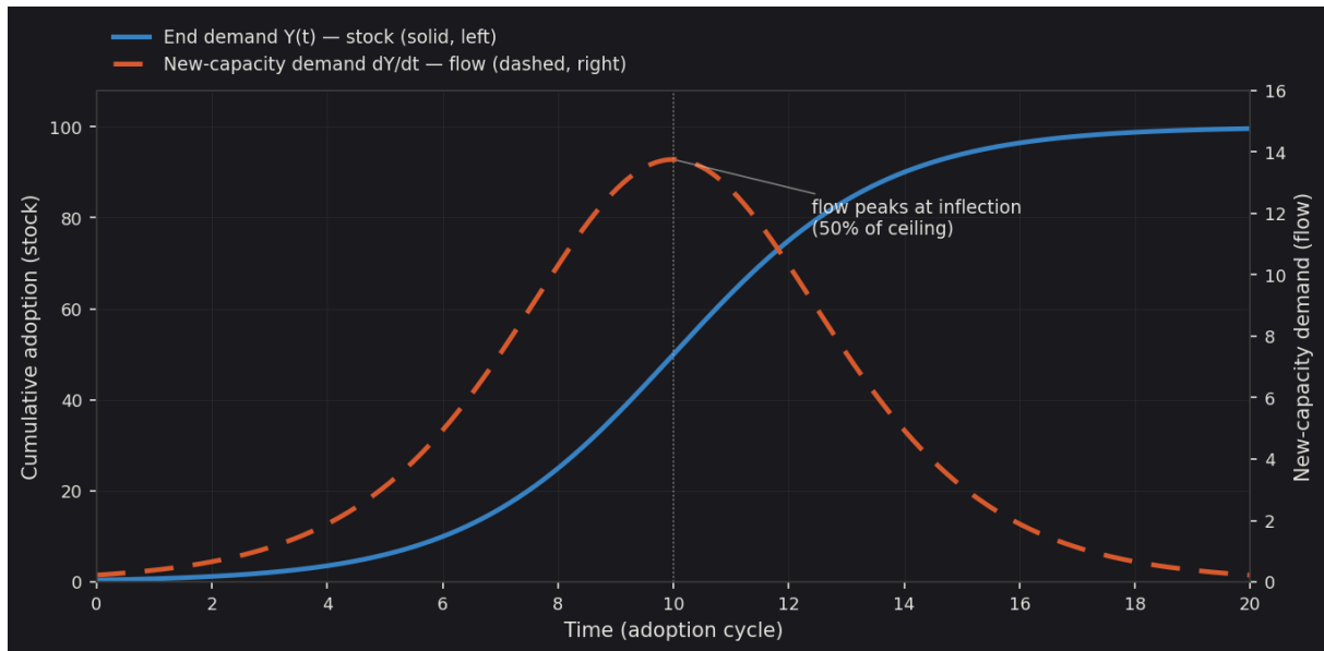
Figure 1: The logistic adoption curve and its derivative
