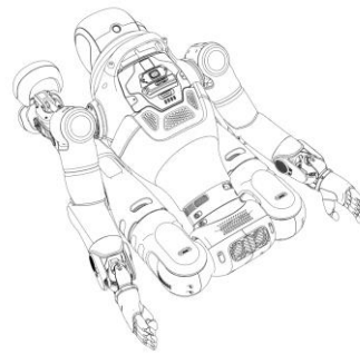
Step1-3: Place in Folded Posture
