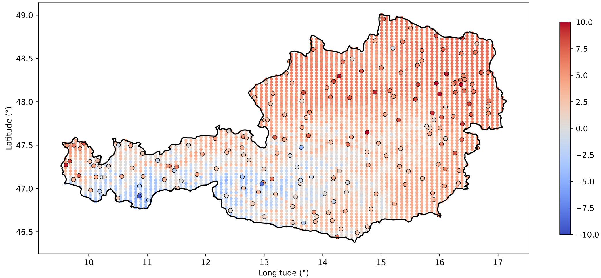
BLR Predictions
