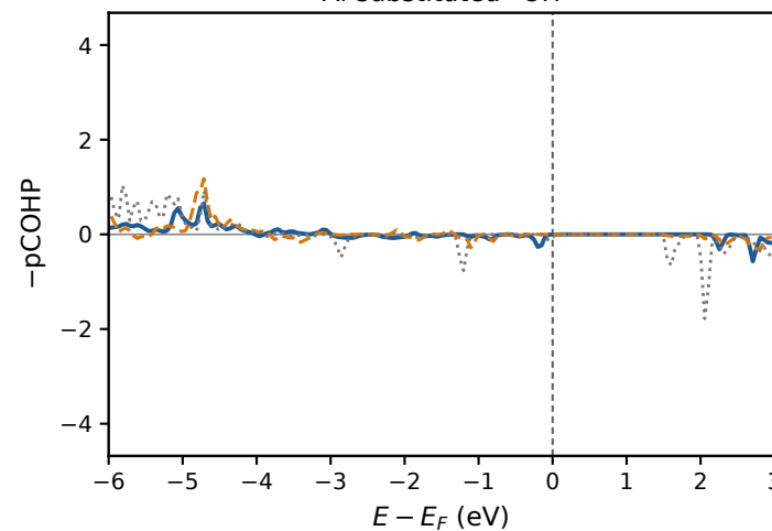
Al-substituted *OH
