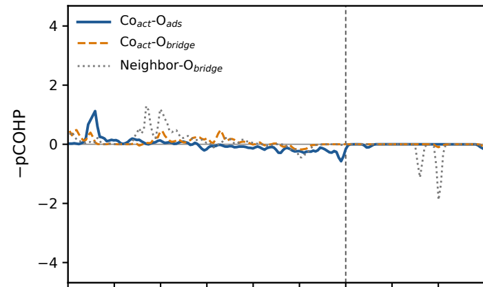
Al-substituted *OH
