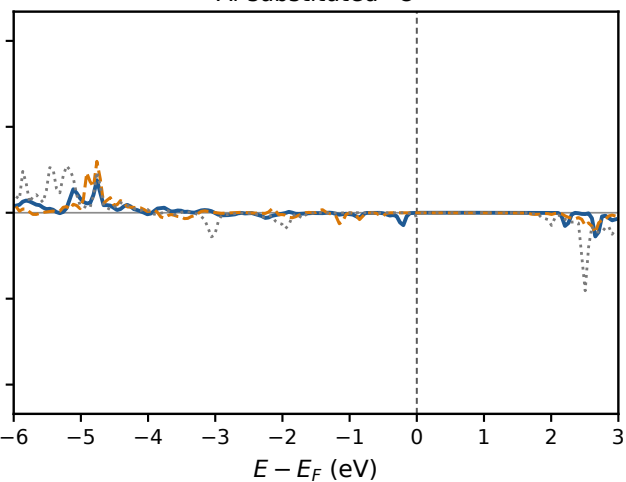
Al-substituted *O
