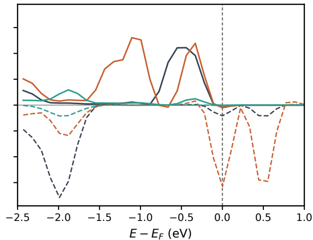
Al-substituted *O
