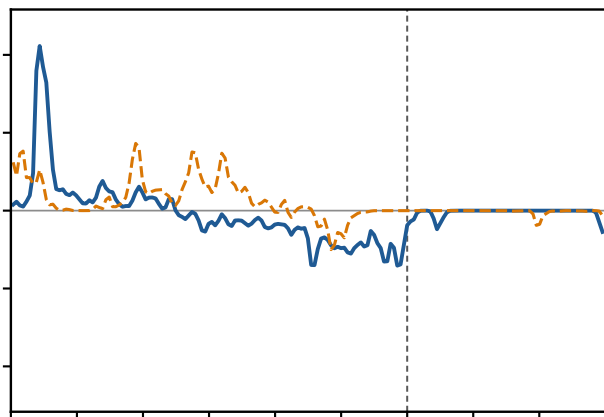
Al-substituted *O
