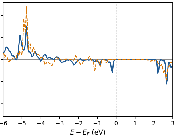
Al-substituted *O
