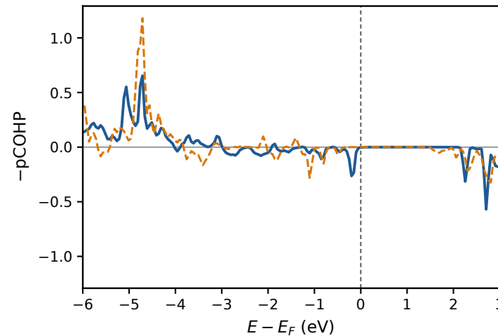
Al-substituted *OH
