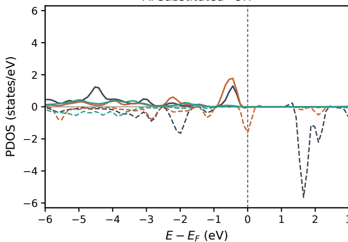
Al-substituted *OH
