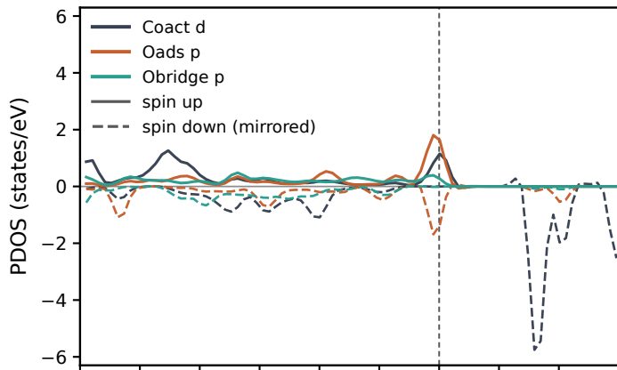
Al-substituted *OH
