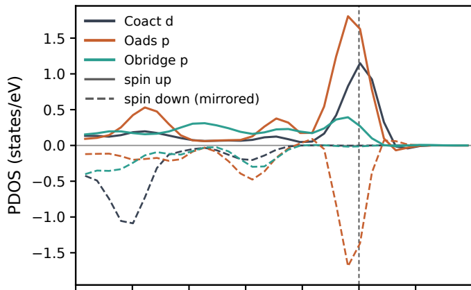
Al-substituted *OH
