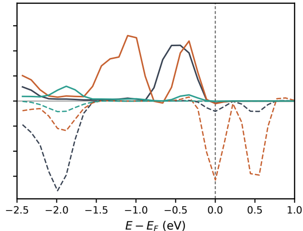
Al-substituted *O
