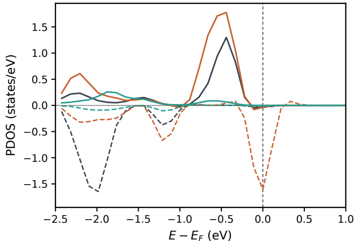
Al-substituted *OH
