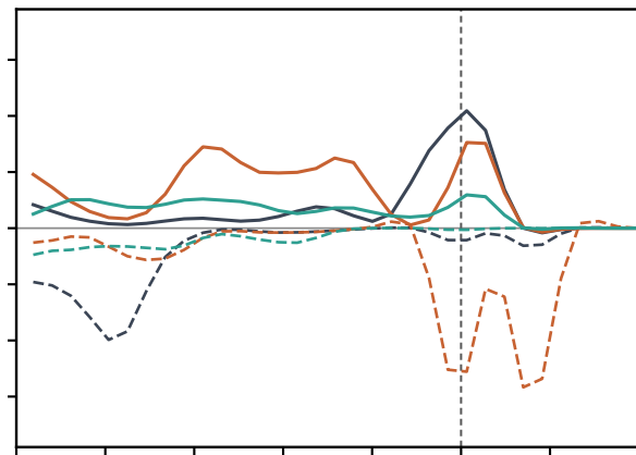
Al-substituted *O
