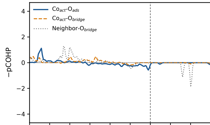
Al-substituted *OH
