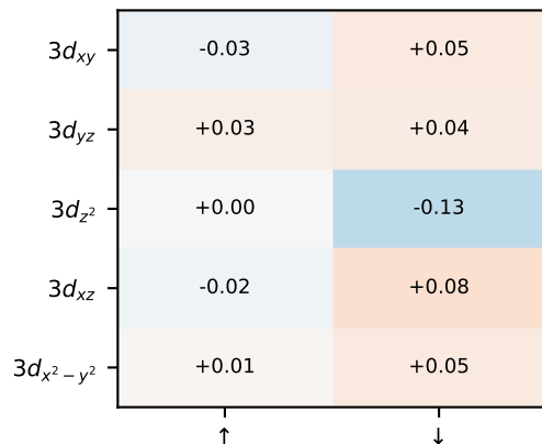
Pristine CoOOH - Co 3d
