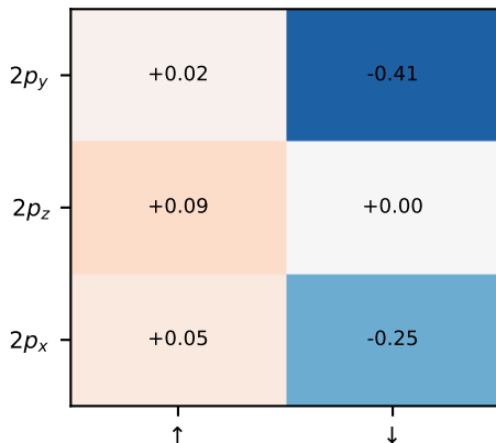
Pristine CoOOH - O ads 2p
