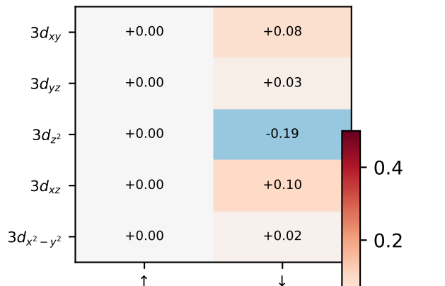
Al-substituted CoOOH - Co 3d
