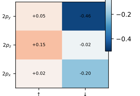
Al-substituted CoOOH - O ads 2p
