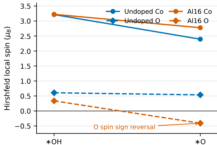
(b) Local-spin evolution
