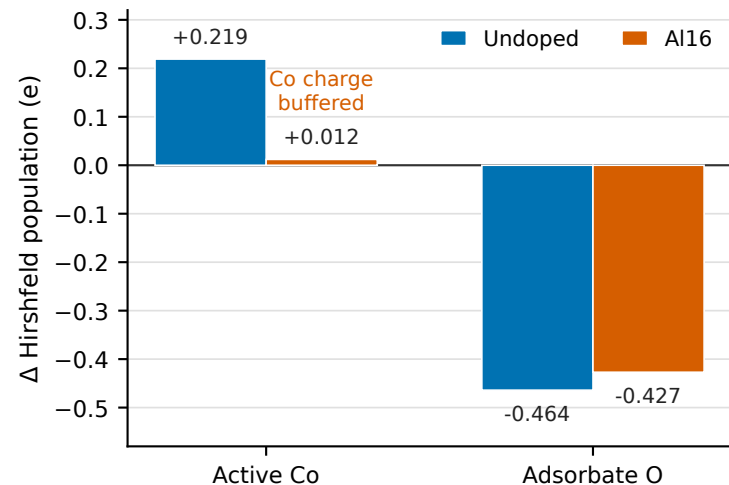
(a) Charge redistribution, *OH → *O
