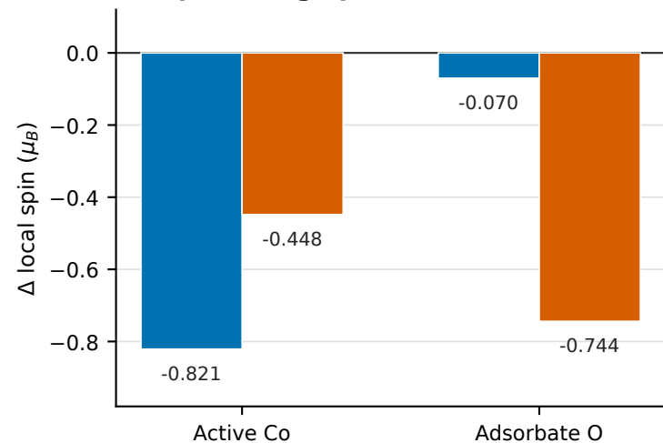
(c) Spin-change partition
