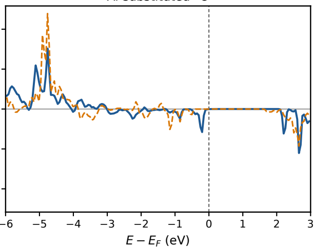
Al-substituted *O
