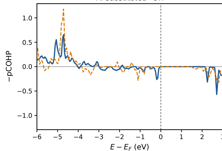
Al-substituted *OH
