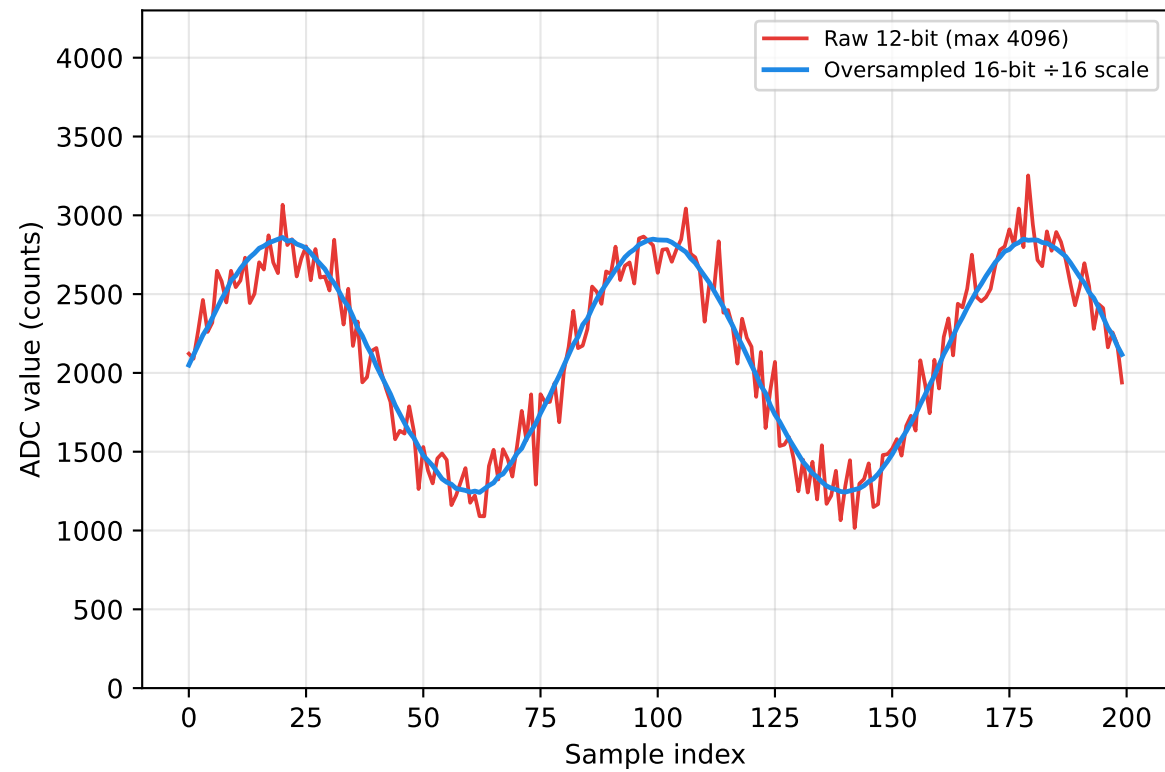
ADC: Raw 12-bit vs Oversampled 16-bit
