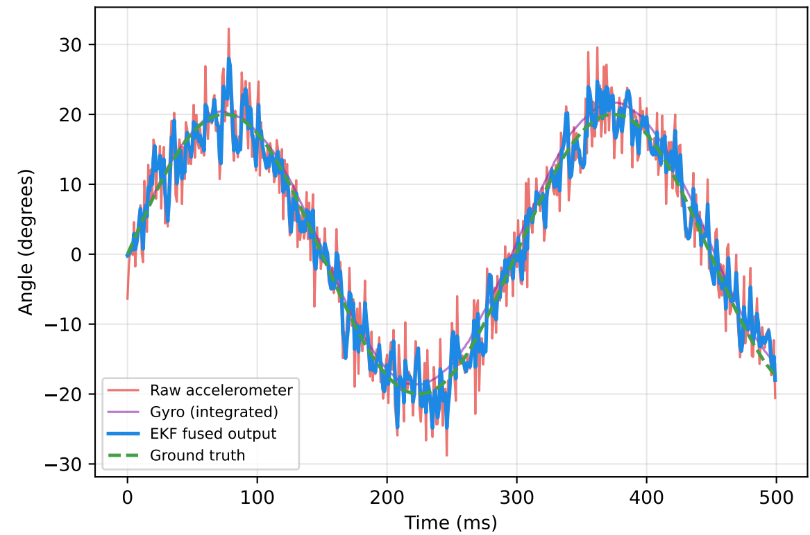
EKF Sensor Fusion — Angle Estimation
