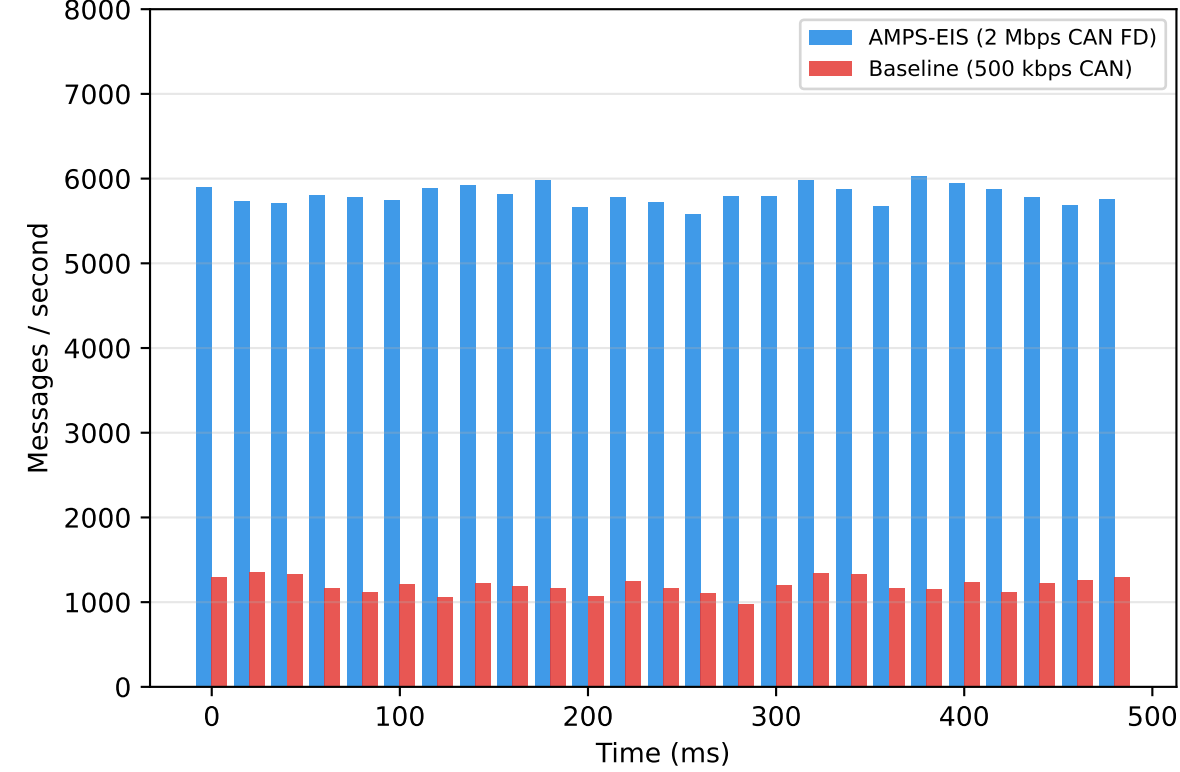
CAN FD Message Throughput Comparison
