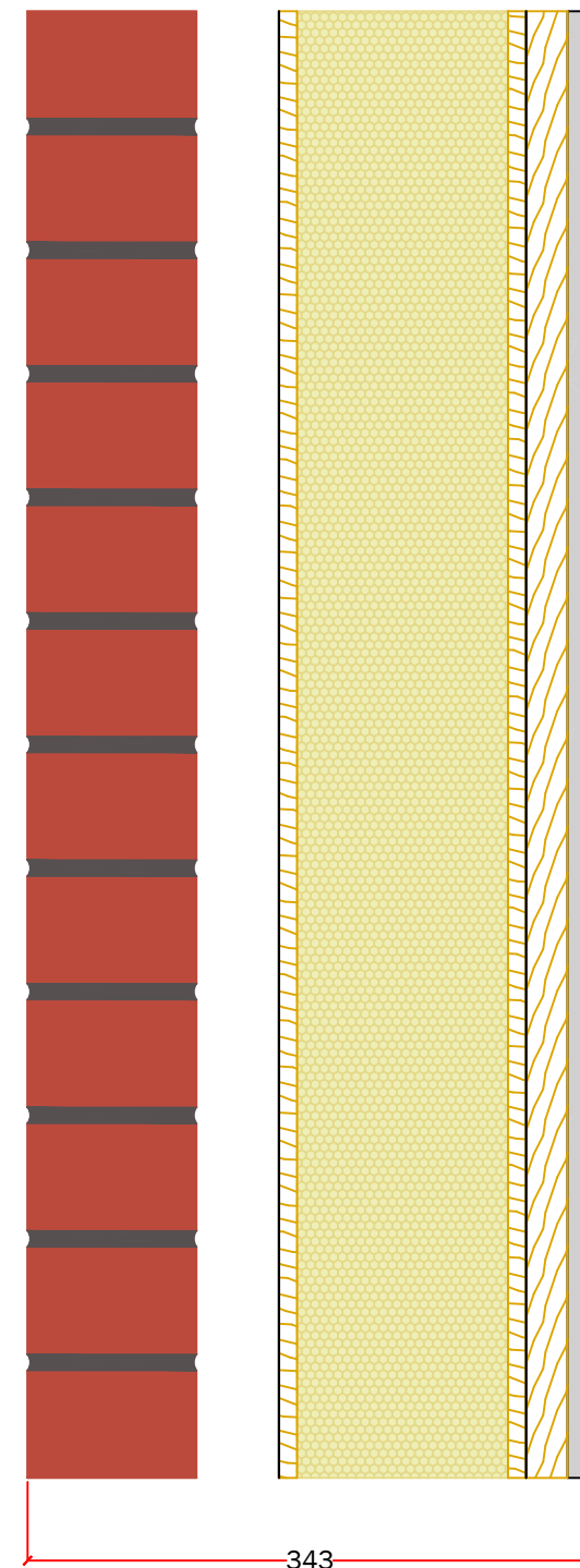
Traditional brick and SIP wall
