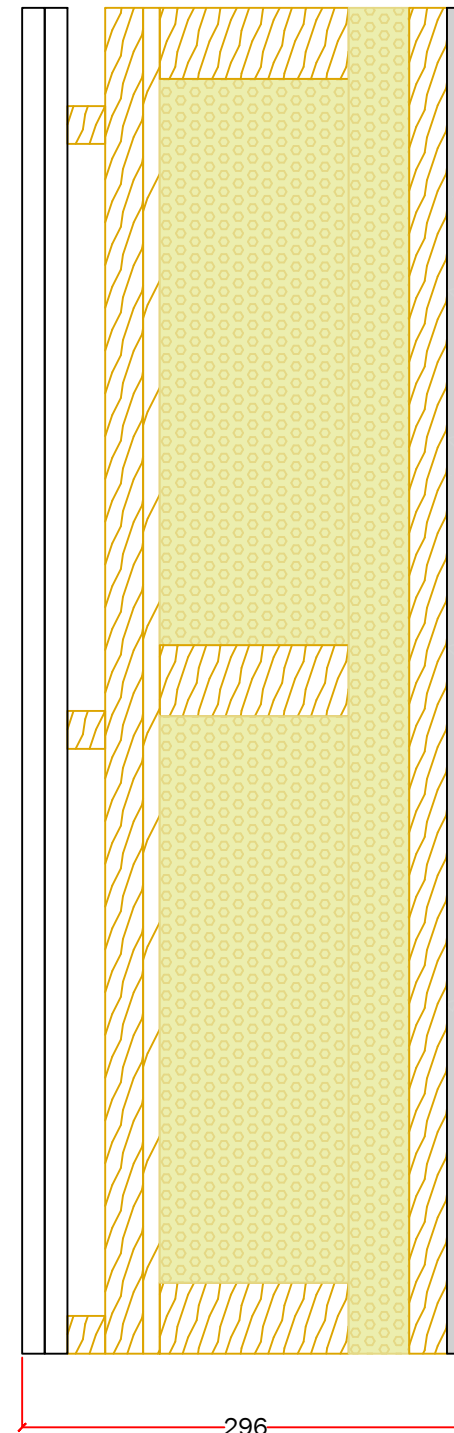
Render onto timber frame wall
