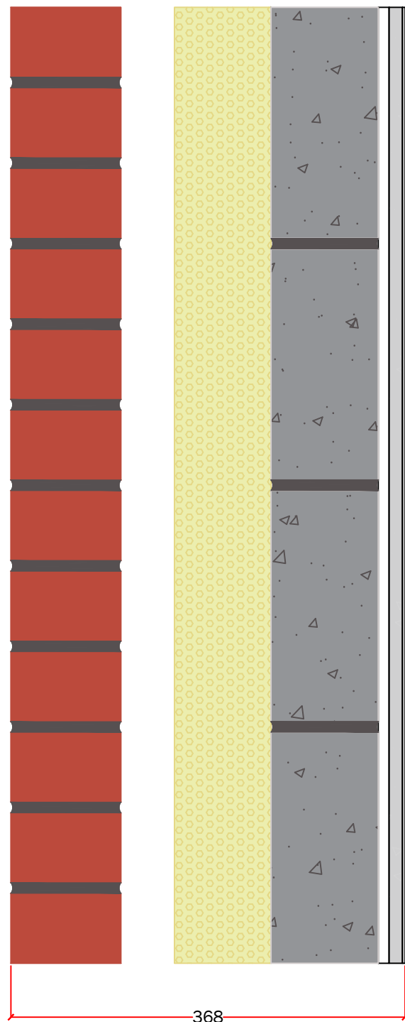
Traditional brick and block wall
