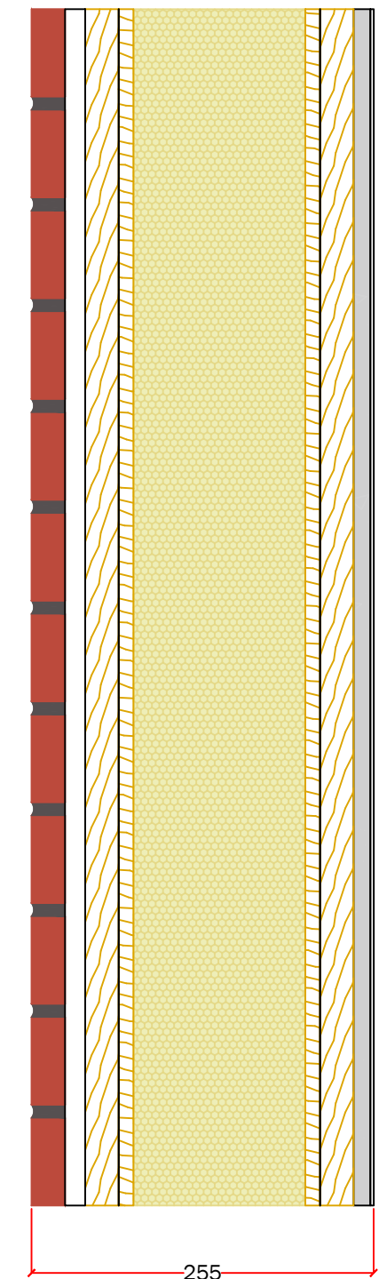
Brick slip and SIP wall
