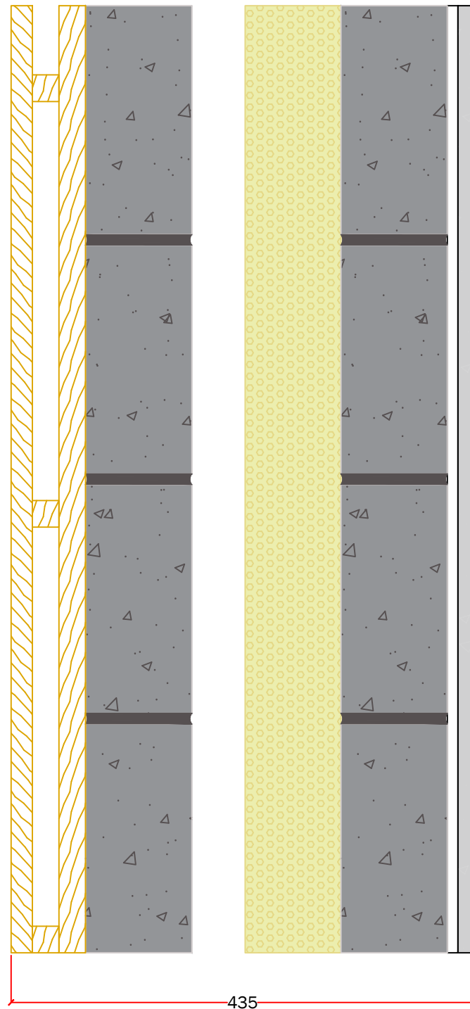
Timber cladding onto block wall
