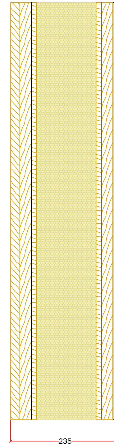
Timber cladding and SIP wall
