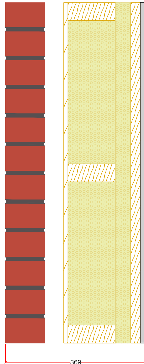
Traditional brick and timber frame wall
