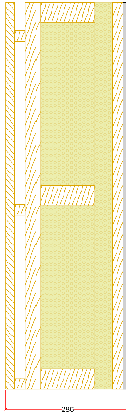
Timber cladding onto timber frame wall
