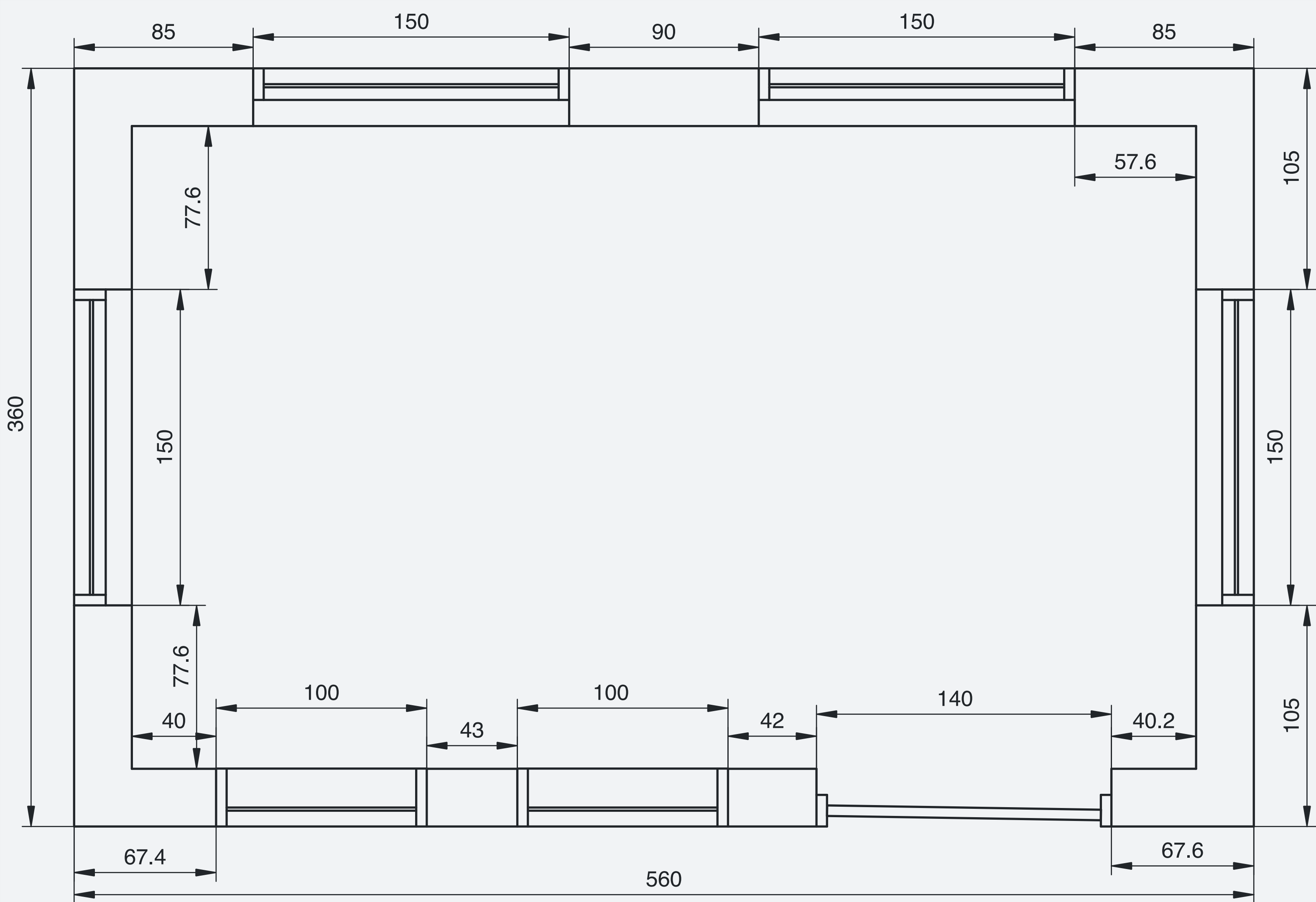
1:15 plan - all measurements in Centimetres
