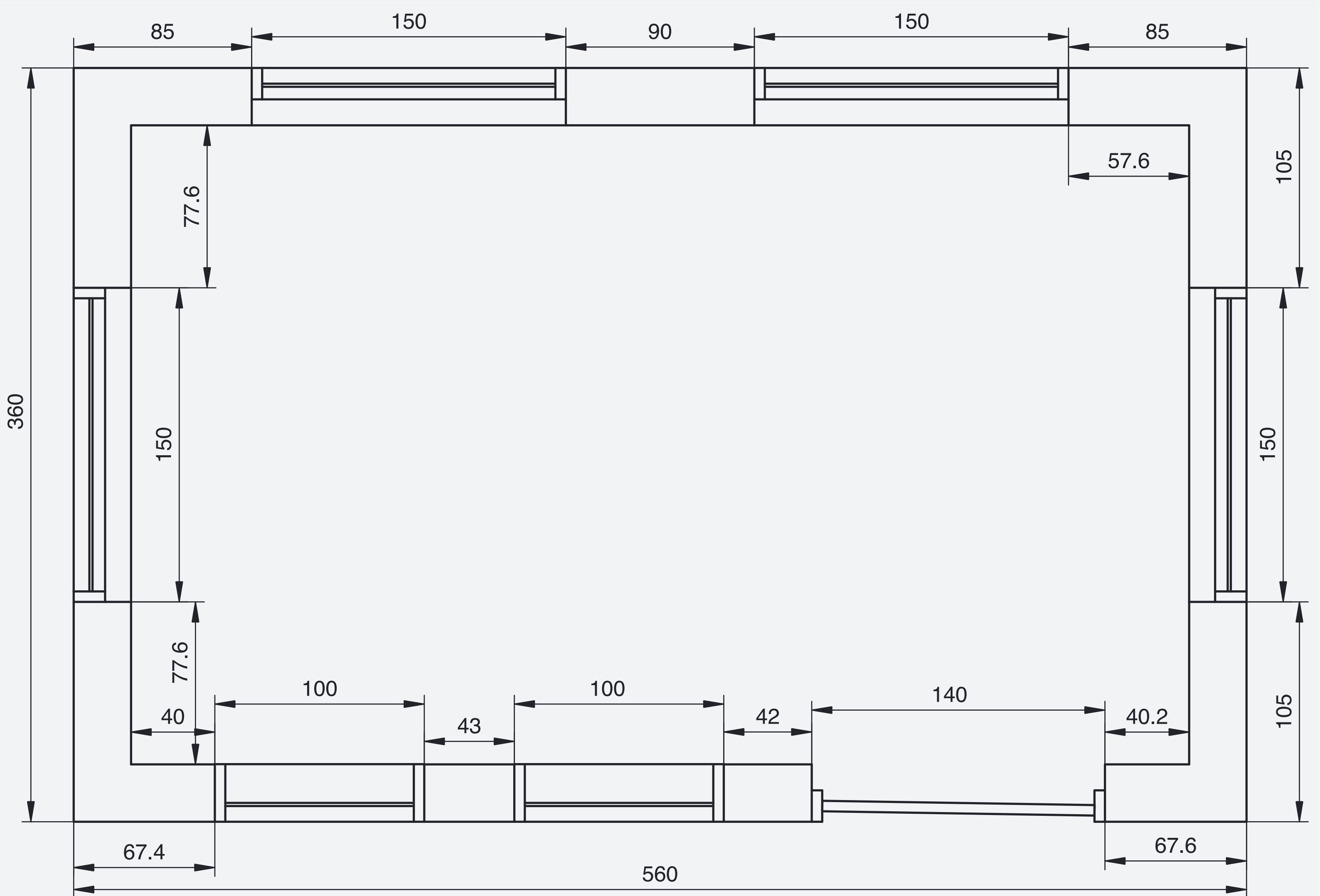
1:15 plan - all measurements in Centimetres
