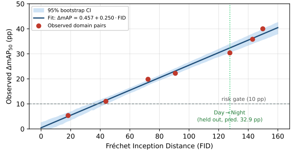
Figure 2: Observed \text{mAP}_{50} degradation versus Fréchet Inception Distance across the seven real domain pairs, with the fitted FID-only predictor and its 95% bootstrap band. The held-out Day→Night pair (prediction 32.9 pp, actual 30.4 pp) is highlighted.
