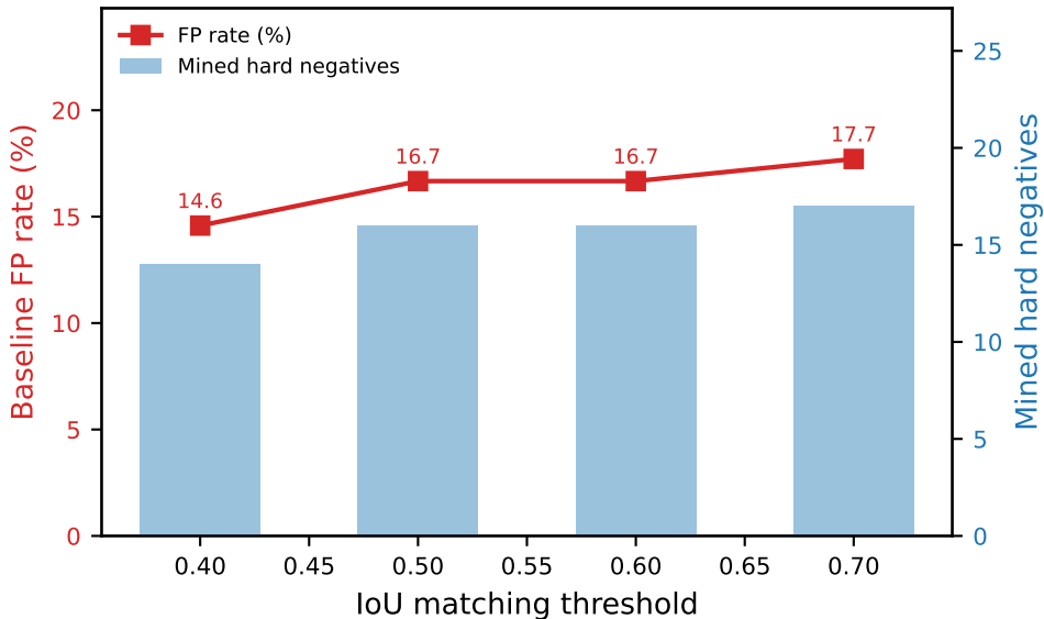
IoU threshold sensitivity (baseline, held-out val)
